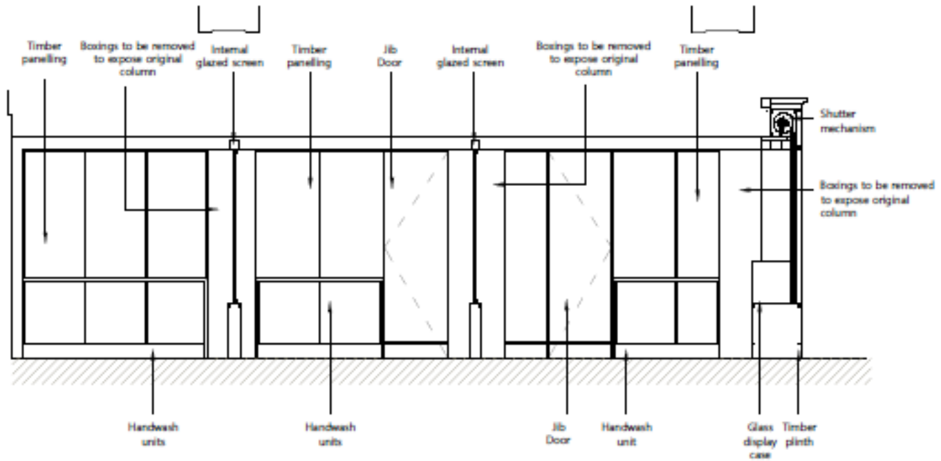
1.0 Internal Elevation
