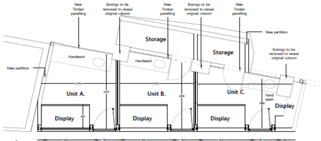
1.0 Plan
